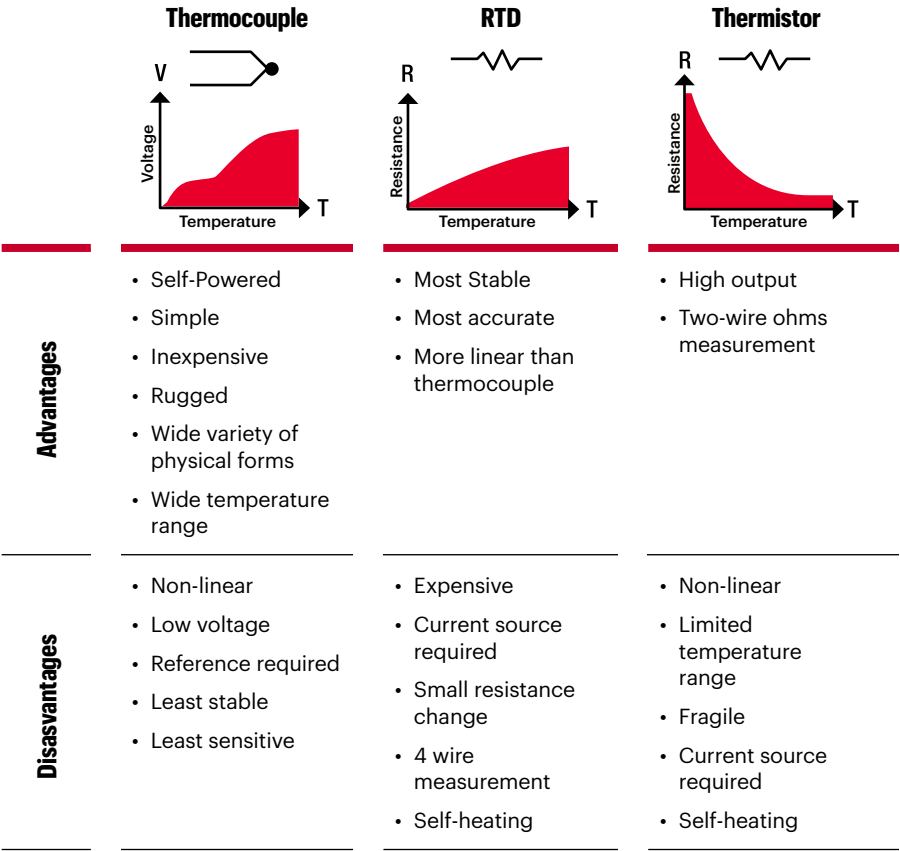
Figure 7. Temperature sensor type comparisons – advantages and disadvantages
